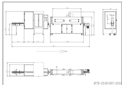
APTB-250B+SST-2500
